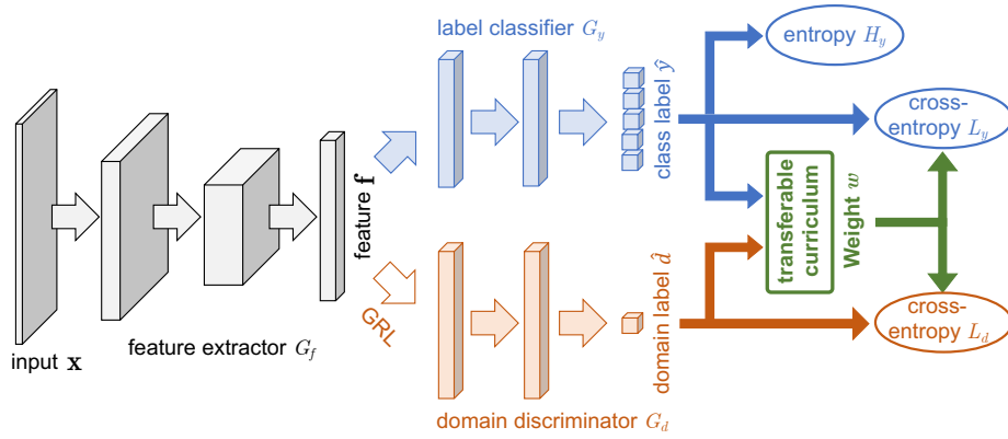
Figure 2: The proposed architecture to learn a transferable curriculum for weakly-supervised domain adaptation. In the diagram, f is the deep feature extracted by a feature extractor G_f , \hat{y} is the class label predicted by a label classifier G_y , and \hat{d} is the domain label predicted by a domain discriminator G_d ; The corresponding losses are L_y , L_d and H_y , and GRL is the Gradient Reversal Layer introduced in (Ganin and Lempitsky 2015) for domain adversarial training. In particular, w is a binary weighting scheme for the transferable curriculum, indicating the selection and timing of each example into training. Best viewed in color.
