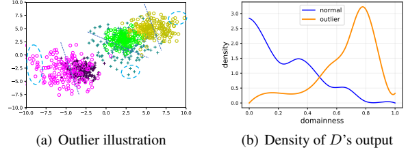
Figure 4. (a) Plot of source ( \circ ) and target ( + ) samples. Dotted lines indicate the best linear classifier to discriminate source from target. The dotted ellipses highlight the outliers. (b) The density of domain discriminator D 's output for normal samples and outliers. The output of D is continuously distributed in the range [0, 1] instead of concentrated on 0 and 1 since source and target samples are not perfectly separable and we use a one-layer classifier. The similar observation is also found in [44].
