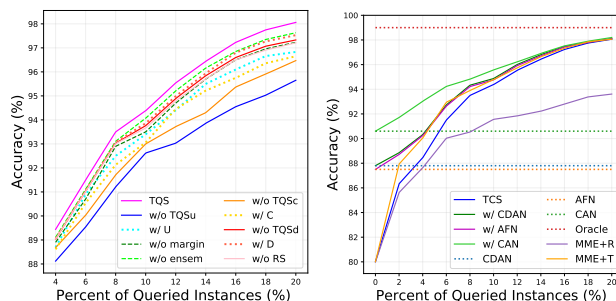
(a) Ablation Study of TQS (b) Combine TQS with UDA/SSDA
