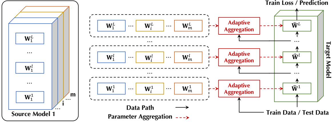
Figure 1. The framework of our proposed method. We derive the target model \widehat{W} by aggregating the parameters of the source models W_i in each layer, controlled by the learnable adaptive aggregation modules based on the input data. During training, the adaptive modules are trained, and the source parameters are tuned to transfer to the target task. After training, the tuned source models are aggregated depending on each query data for inference.
